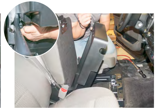
Lift the plastic base from the center console, being careful to disconnect the wires from the rear of the base.
