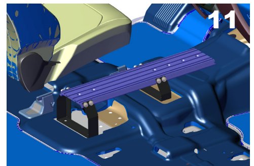
Place the Floor Plate in desired location by sliding forward and back. Secure by tightening the 5/16 nuts.
