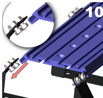
Lightly secure (8) of the 5/16-18 bolts, washers, and nuts to the Floor Plate Brackets. Slide the Floor Plate in from the rear, aligning the bolts with the side grooves on the Floor Plate side.
