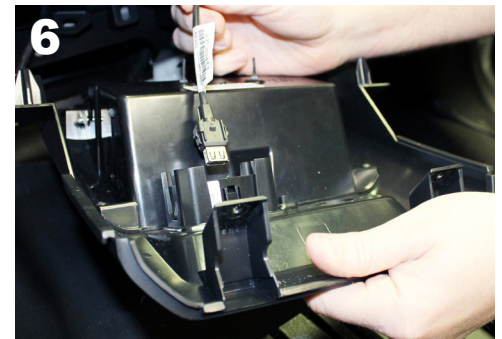
Unclip USB cable from dash port. Trace the cable back and find where it is tied to the wiring harness. Free the attached point to allow enough cable length for relocation of USB.
