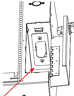
Remove lower panel containing 12 volt power and USB by unscrewing (2) 7mm screws on the top and (2) 10mm screws on the bottom. Unplug accessories from harness.
