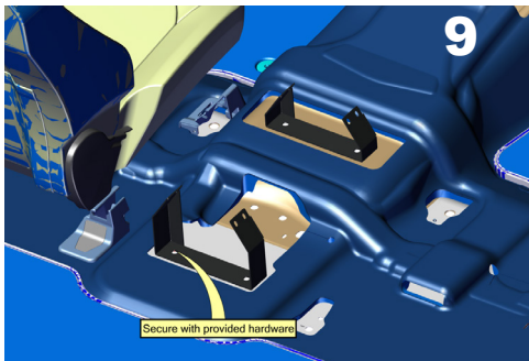
Place front and rear Floor Plate Brackets over hole locations. Secure with provided bolts or OEM hardware.
