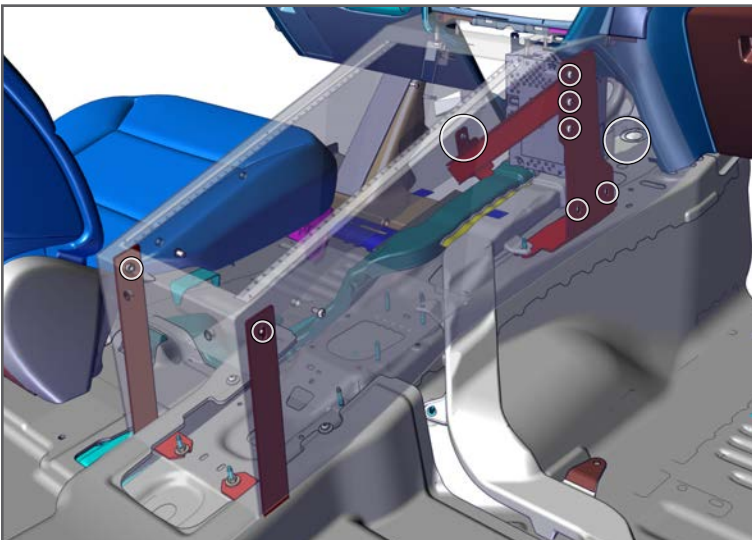
8. With the radio moved aside secure the front hole with provided self-drilling screw.
