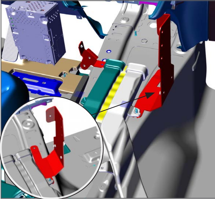
7. Attach the P/S front bracket by detaching the OEM radio and moving it to the left. Secure the D/S front brackets rear mounting hole to the stud, under the air ducts mounting tab with previously removed 10 mm nut, and front mounting hole with provided hex head tapping screw.
